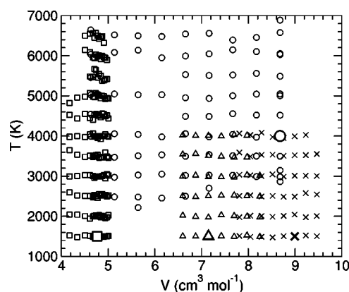
FIG. 1. Location of points in the V - T plane at which we conduct simulations of the liquid (circles), stishovite (squares), coesite (triangles), and \beta -quartz (crosses). The large symbols locate reference states (V_R, T_R) at which the entropy of each phase is evaluated directly.
