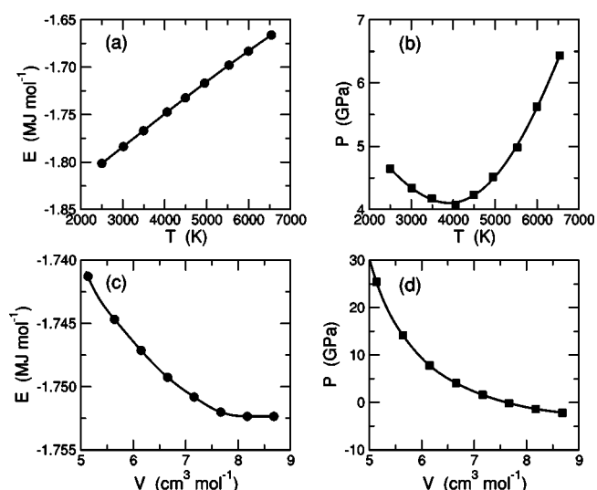
FIG. 2. Examples of fitted and interpolated data for the liquid phase: (a) values of E along the V=6.655 \text{cm}^3 \text{mol}^{-1} isochore, fitted with a cubic polynomial (line); (b) values of P for V=6.655 \text{cm}^3 \text{mol}^{-1} , fitted with a quartic polynomial (line); (c) interpolated values of E along the T=4000 K isotherm, fitted with a cubic spline (line); (d) interpolated values of P for T=4000 K, fitted with a cubic spline (line).
