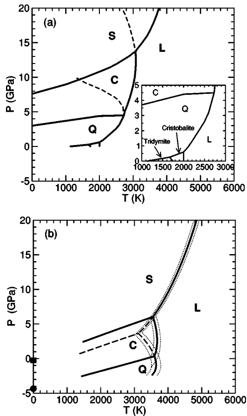
FIG. 5. (a) Experimentally determined coexistence lines of silica in the P - T plane. Stability fields for the stishovite ( S ), coesite ( C ), \beta -quartz ( Q ), and liquid ( L ) phases are shown. Both stable (solid) and metastable (dashed) coexistence lines are shown. The inset shows the stability fields of cristobalite and tridymite, not considered in this work. Adapted from Ref. [3]. (b) Phase diagram of BKS silica in the P - T plane. Solid lines are stable coexistence lines. Dotted lines show error estimates for the crystal-liquid coexistence lines, as described in the text. Metastable coexistence lines (dashed) are also shown that meet at the metastable S - L - Q triple point. The locations of the S - C (filled square) and C - Q (filled circle) coexistence boundaries at T=0 , determined from Fig. 4(b), are also shown.
